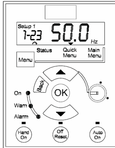
LCP 12 with Potentiometer
